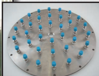
▲ BUBBLER TOP PLATE: produced using the Mazak.
